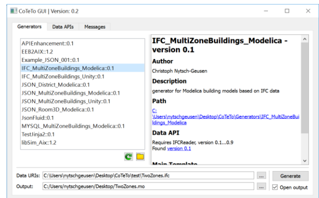
Figure 2. CoTeTo GUI for template based code generation
